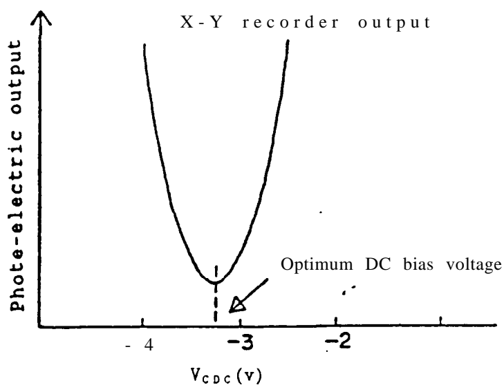
Fig.D Optimum common electrode DC bias voltage by measurement of contrast
