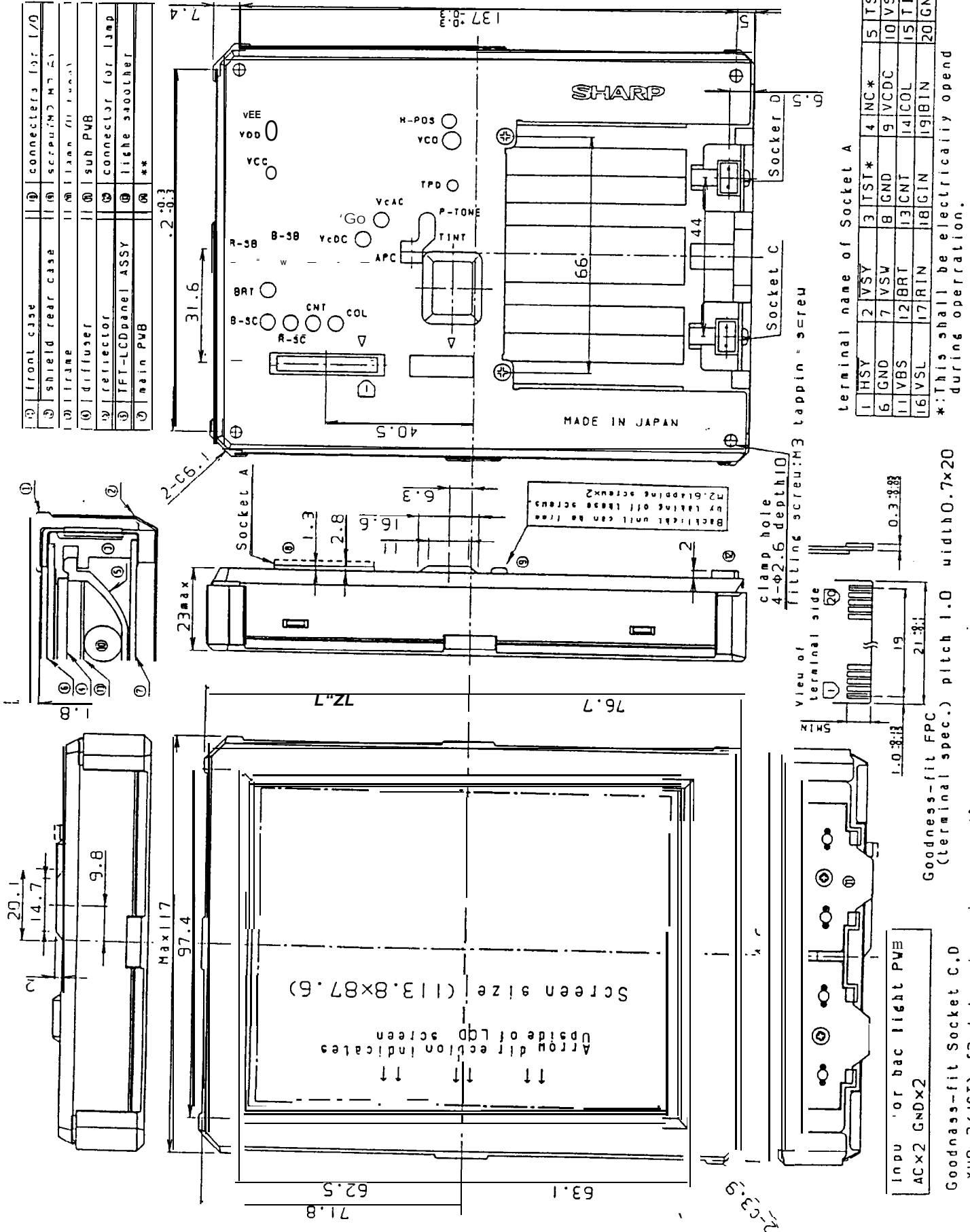
Fig. 3 Out line dimensions of TFT-LCD module
